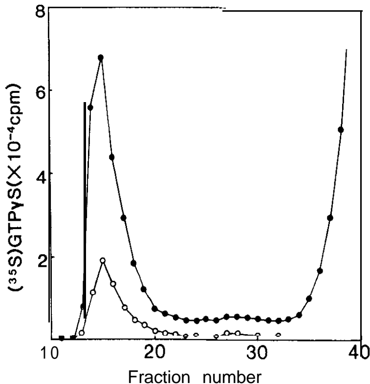
Fig. 2. Gel filtration through a Sephadex G-100 column of crude extract containing membrane components binding [ 35 S]GTPYS. Radioactivity counting in 0.4 ml of each fraction (--*--*) and those retained on membrane filter after washing by the buffer (--O--).
