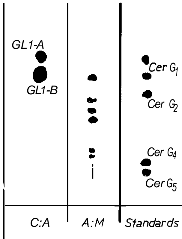
Figure 1. Thin layer chromatography (Silica gel G, Merck) of lipids in fractions C:A and A:M from a silicic acid column. The solvent was chloroform:methanol:water (65:25:4, v:v:v). The plate was stained with the orcinol reagent. CerG 1 , CerG 2 , CerG 4 , and CerG 5 , standards of mono, di, tetra and pentahexosyl ceramide (Supelco).
