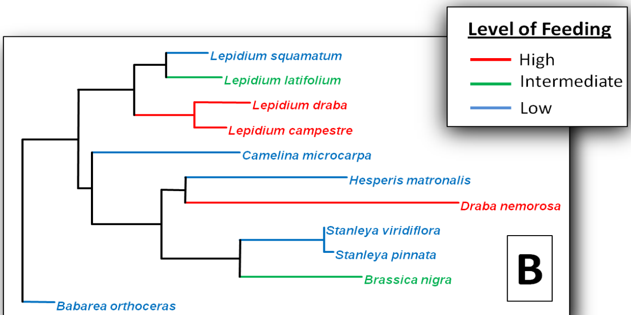
Figure 2. Phylogeny developed from genetic data (A) and the same phylogeny overlaid with Ceutorhynchus cardariae Korotyayev feeding intensity classes (B).
