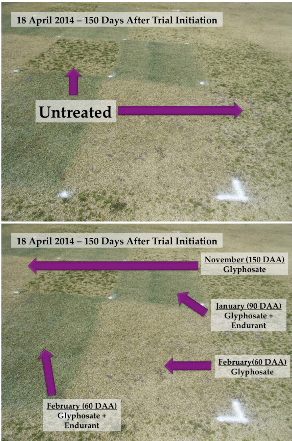
Figure 2. Top: Annual bluegrass populations present in untreated areas, 150 days after trial initiation. Bottom: Effective annual bluegrass control with glyphosate and glyphosate + Endurant applications in November, January, and February.
