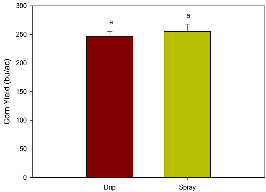
Figure 4. Corn grain yield under Mobile Drip Irrigation and in-canopy spray nozzles for well capacity of 600 gpm during the 2015 growing season at the Kansas State University Southwest Research-Extension Center, near Garden City, Kansas.
