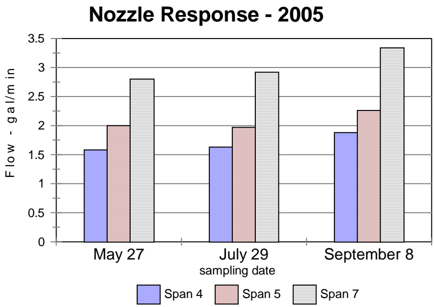
Figure 6. Nozzle response from 2004 and 2005.
