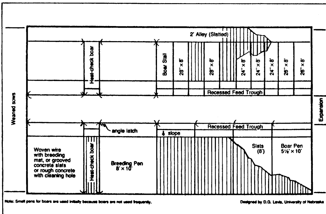
Figure 3. Breeding facility with built-in expansion.
