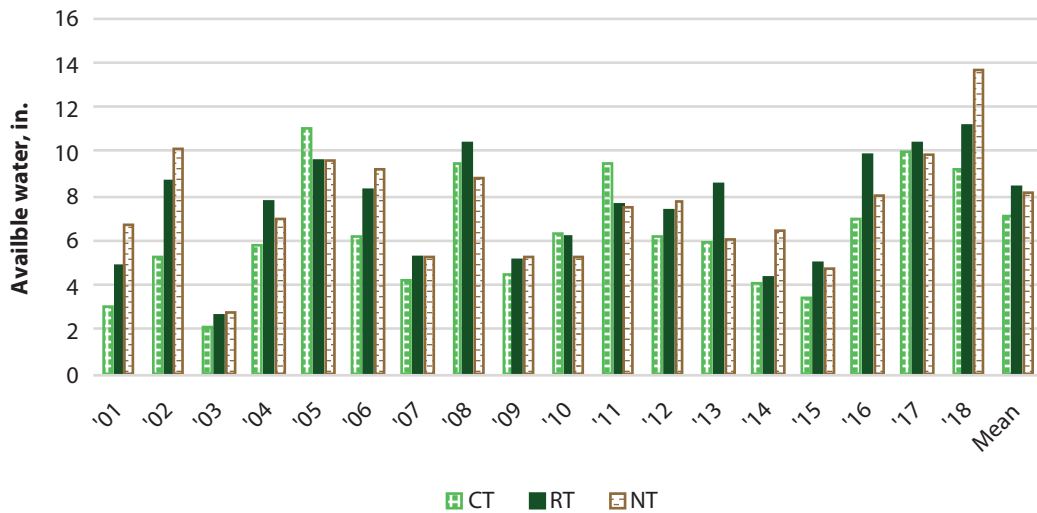
Figure 1. Available soil water in 8-ft profile at planting of wheat in a wheat-sorghum-fallow rotation as affected by tillage intensity, Tribune, KS, 2001–2018. The last set of bars (Mean) is the average across years. CT = conventional tillage. RT = reduced tillage. NT = no-tillage.
