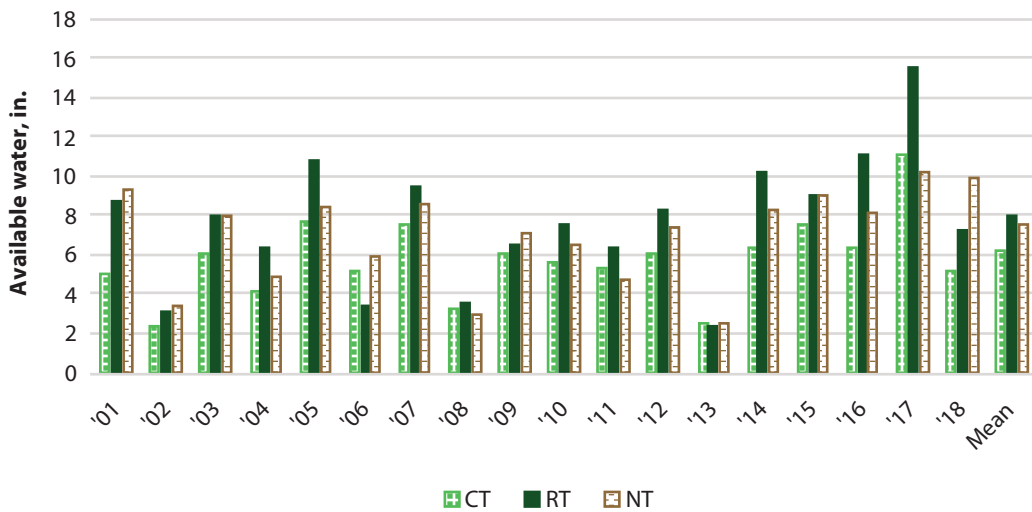
Figure 2. Available soil water in 8-ft profile at planting of grain sorghum in a wheat-sorghum-fallow rotation as affected by tillage intensity, Tribune, KS, 2001–2018. The last set of bars (Mean) is the average across years. CT = conventional tillage. RT = reduced tillage. NT = no-tillage.
