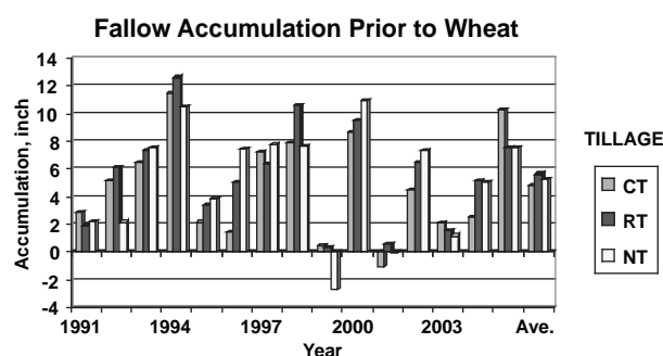
Figure 1. Soil water accumulation during fallow before wheat in a WSF rotation, 1991-2005, Tribune, Kan.
