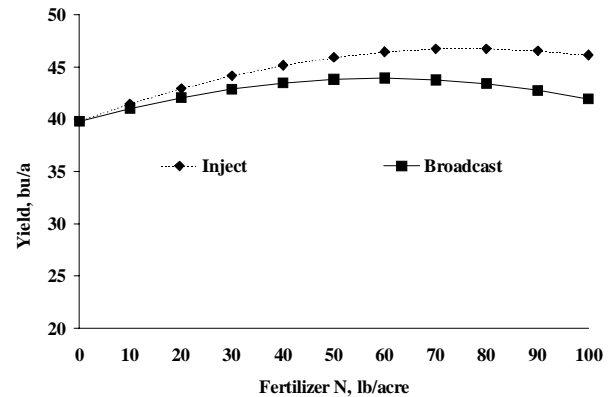
Fig. 5. Estimated wheat yields for injected and broadcast N fertilizer applications with residual soil nitrate content of 75 lb/acre, west central Kansas.
